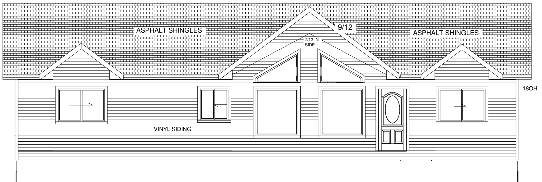
REAR ELEVATION
