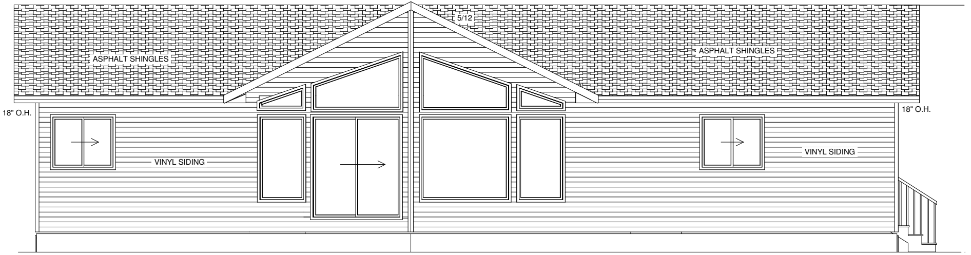
REAR ELEVATION
