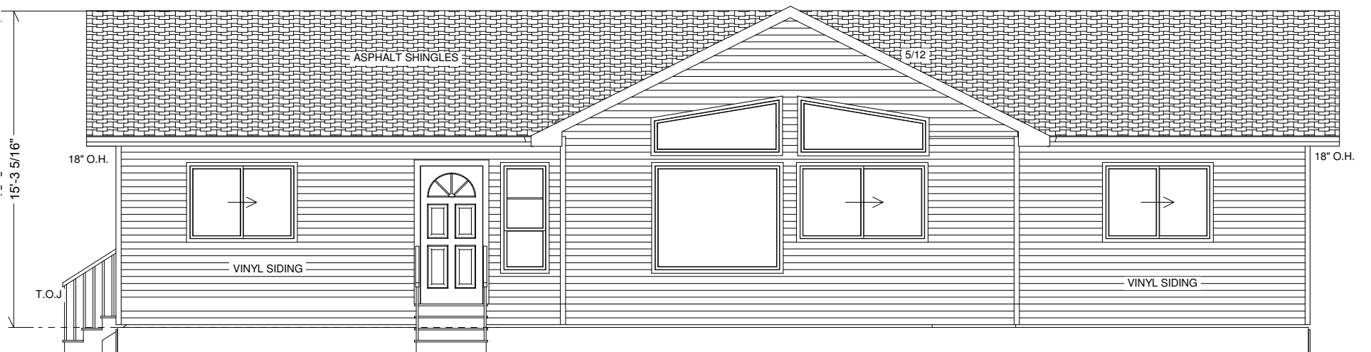
FRONT ELEVATION
